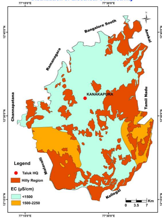
Fig.14: Distribution of EC
