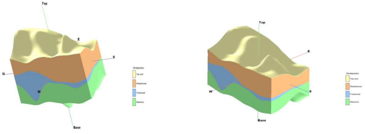
Fig.13b:3D AQUIFER DISPOSITION
