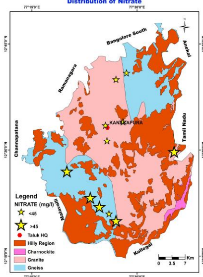
Fig.16: Distribution of Nitrate
