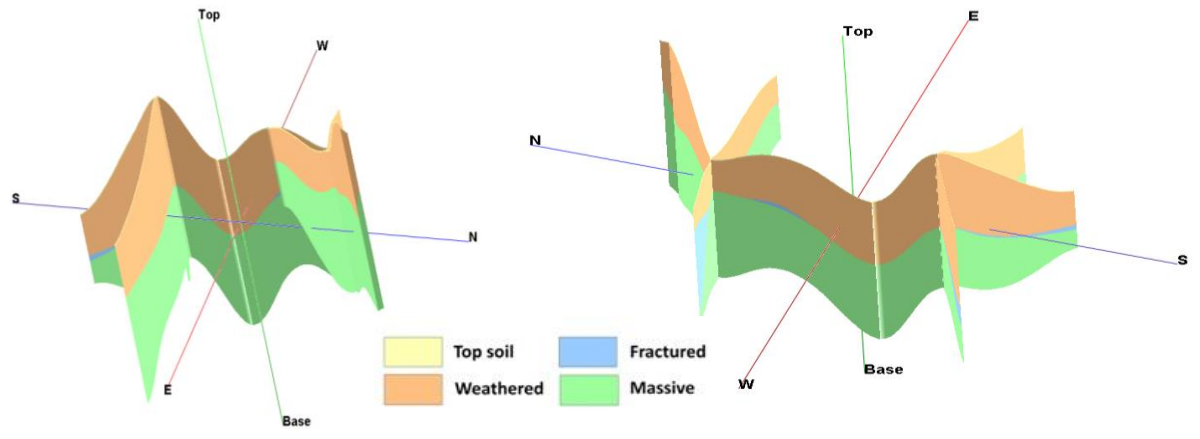
Fig.13c:3D AQUIFER Fence diagram
